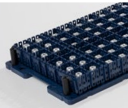
Basic plate in Schäfer-2 format
